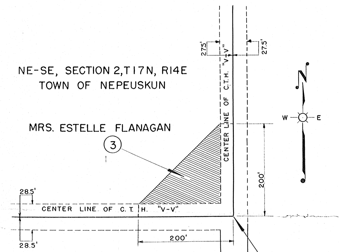
PLAN OF PARCEL NO. 3
