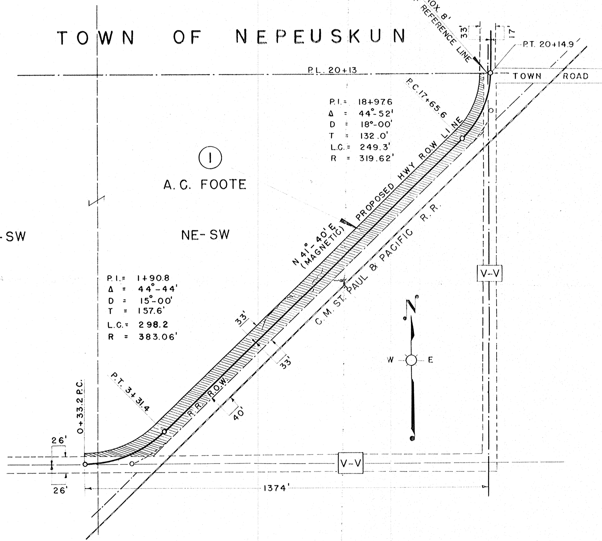
PLAN OF PARCEL NO. 1
