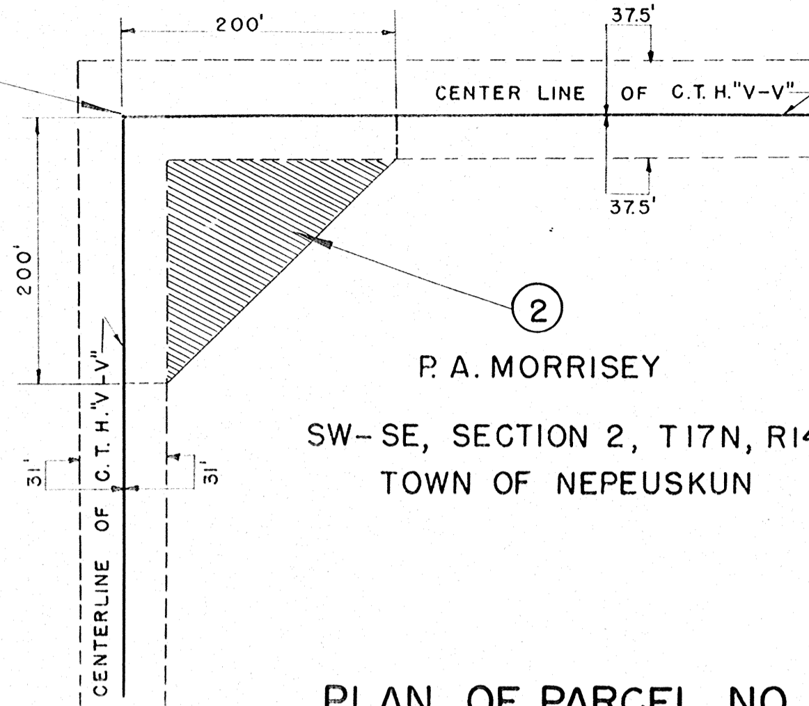
PLAN OF PARCEL NO. 2
